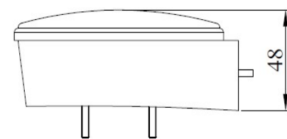
LED Combination Front Lamp
